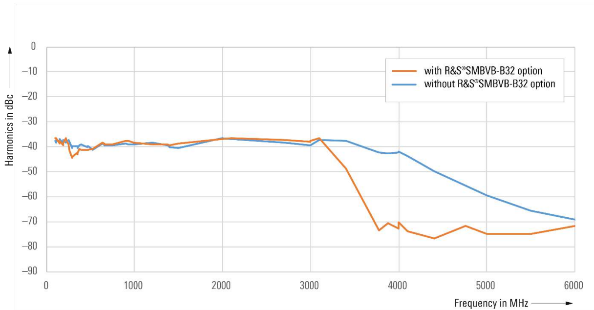
Measured harmonics second order, CW, level = +13 dBm
