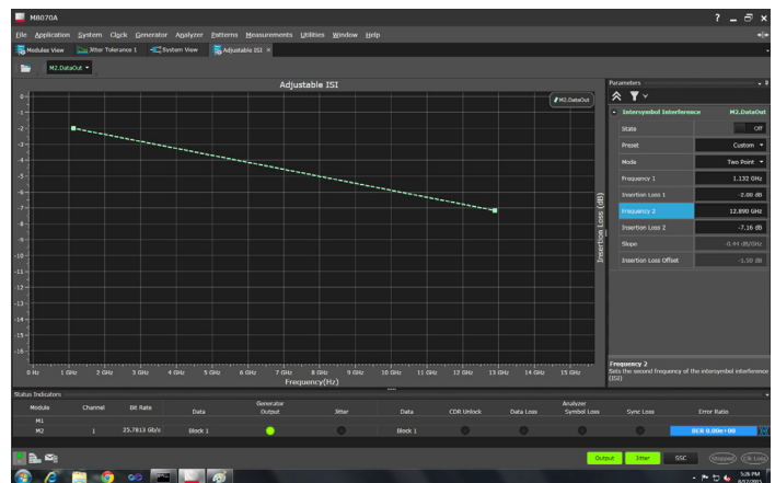
Figure 3. Control ISI for channel emulation is simply entering loss and frequency breakpoints, or by Importing S-parameters.
