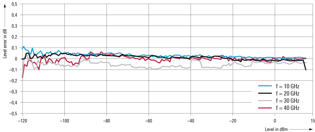
Level linearity with R&S®SMB-B140 and R&S®SMB-B32 options, ALC on (meas.).
