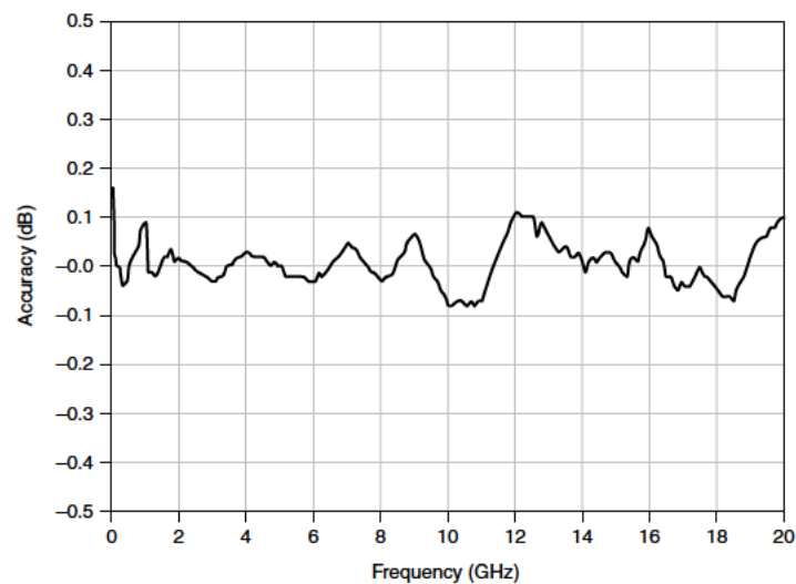
Figure 8 : PXIe-5654 with PXIe-5696 Typical Power Accuracy at -40 dBm
