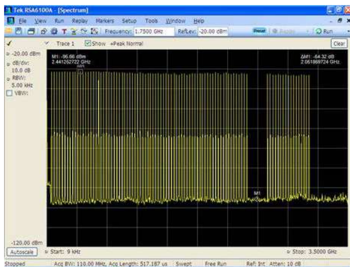
3 GHz wide multi-carrier signal generated on the AWG70000B with over 60 dBC SFDR
