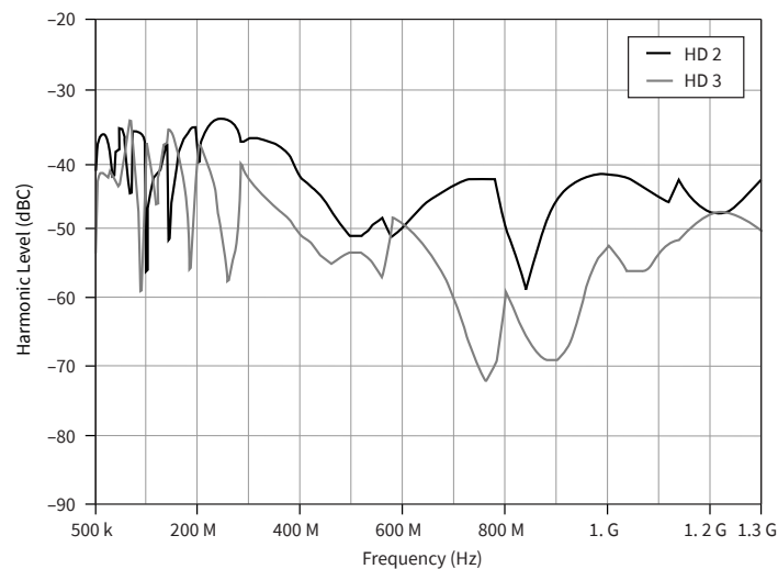
Figure 3. Typical Second Harmonic (HD 2) and Third Harmonic (HD 3) Levels (0 dBm Output Power)
