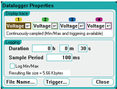
Figure 7. To set up the data logger, use a menu screen to select the operating parameters. Setup screens like this are used throughout the DC power analyzer.
