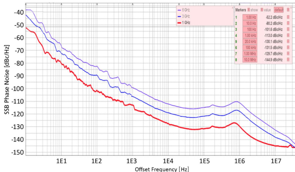
Figure 2. Typical phase noise
