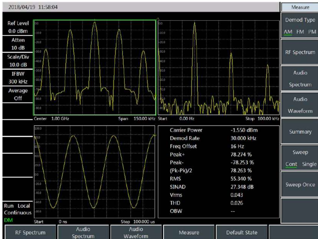
AM/FM/PM Analyzer
