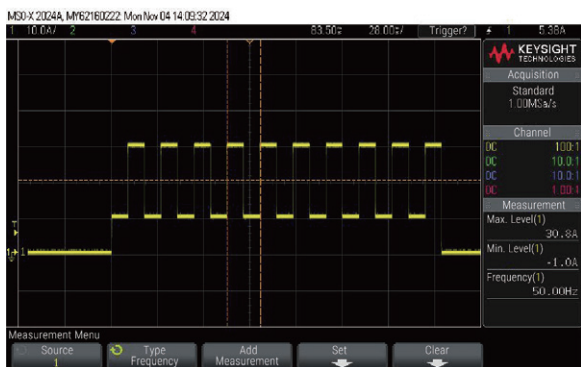
▲ Dynamic current waveform
