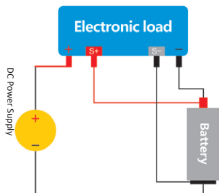
▲ Charge Wiring
