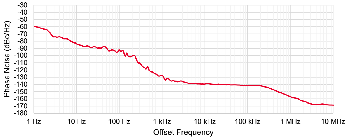
Measured SSB Phase Noise of Auxilliary Fixed LO at 9.6 GHz (options M9484C-AL2, M9484C-600)
