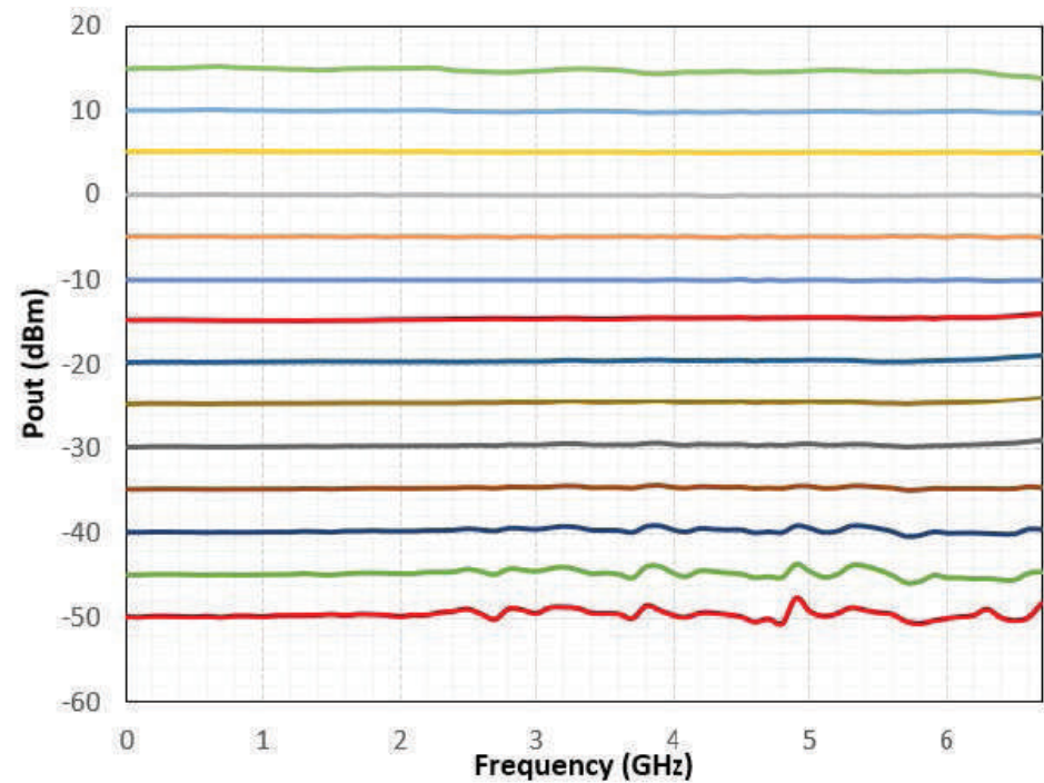
Figure 2: · Calibrated Output Power · -50 dBm to +15 dBm · 10 MHz - 6.0 GHz
