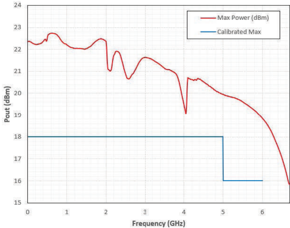
Figure 1: · Maximum Output Power · 25 dBm Setting · 10 MHz - 6.0 GHz
