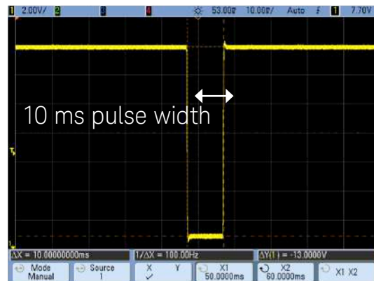
Figure 4. Voltage interrupt pulse generated by N7951A
