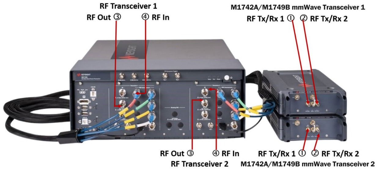
Figure 3. S9110A-TR2/TN2 (with F32, F43 or F49 options) 5G Multi-Band Vector Transceiver configuration 1
