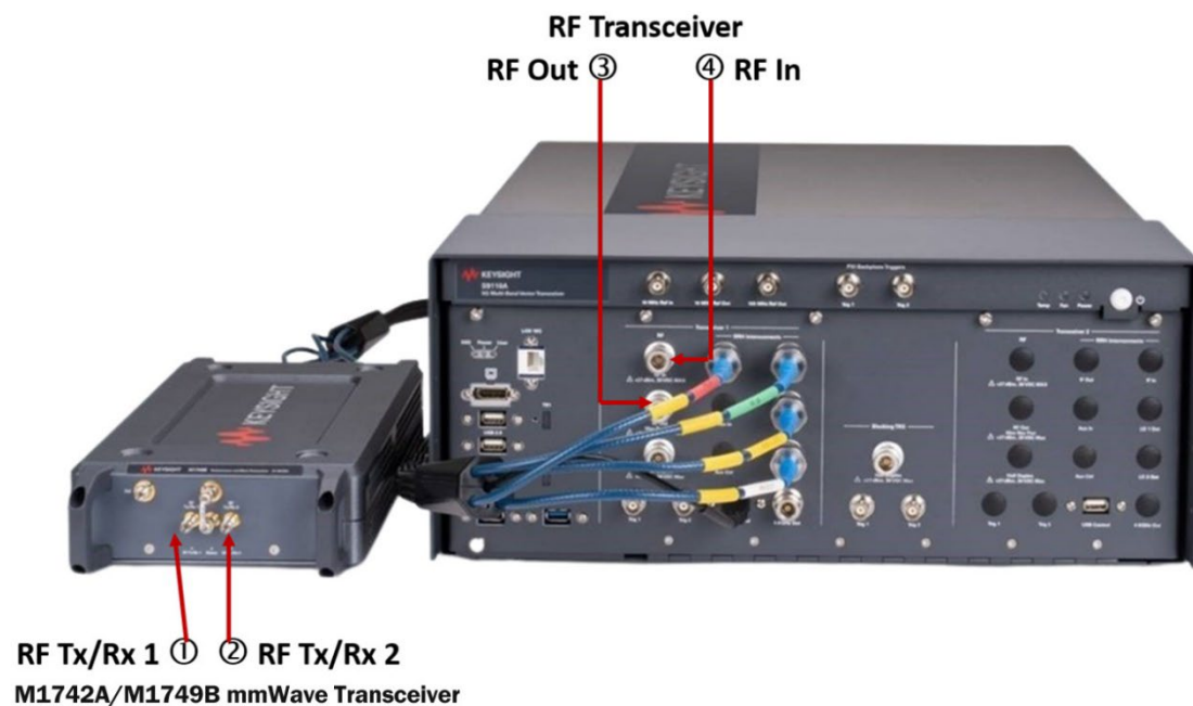
Figure 1. S9110A-TR1/TN1 (with F32, F43 or F49 options) 5G Multi-Band Vector Transceiver configuration 1
