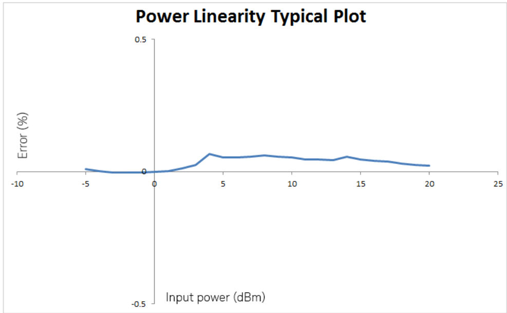
Figure 1. Typical U8480 Series power linearity at 25 °C with measurement uncertainty of ± 0.21%
