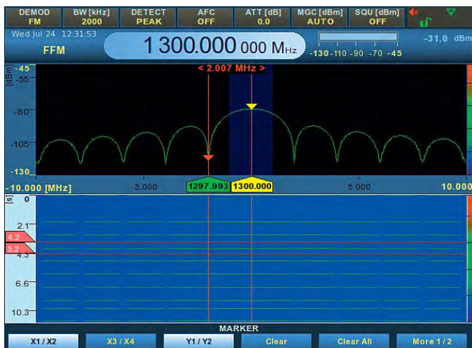
Short-term signals are clearly displayed in the waterfall diagram for easy identification by the user.
