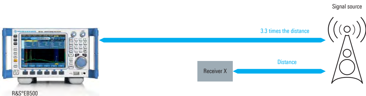
R&S®EB500
