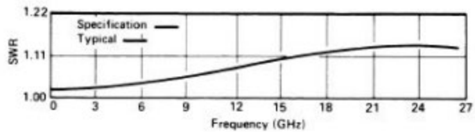
Figure 13. 11667B Leveling or ratio measurement source match (typical)
