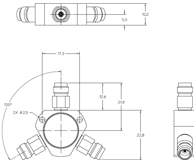
Figure 22. 11667C/D mechanical dimension
