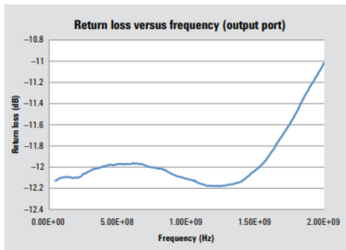
Figure 7. 11667L output port return loss versus frequency (typical)
