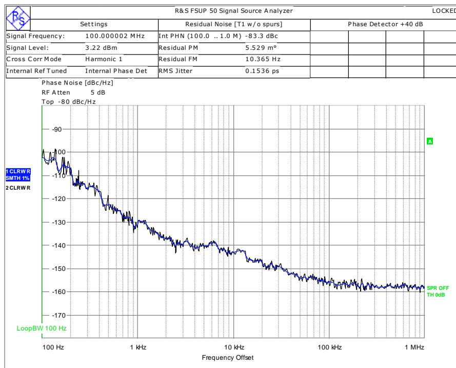
Measured phase noise of wideband analog I/Q outputs; single-ended sine wave with f = 100\text{ MHz}
