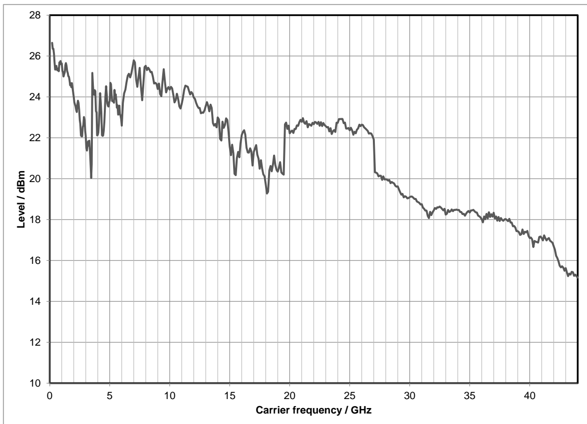
Measured maximum available output level versus frequency with R&S®SMW-B1044, R&S®SMW-B1044N, R&S®SMW-B2044, R&S®SMW-B2044N frequency options
