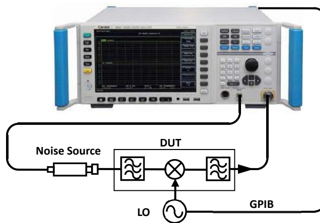
Measurement Setup
