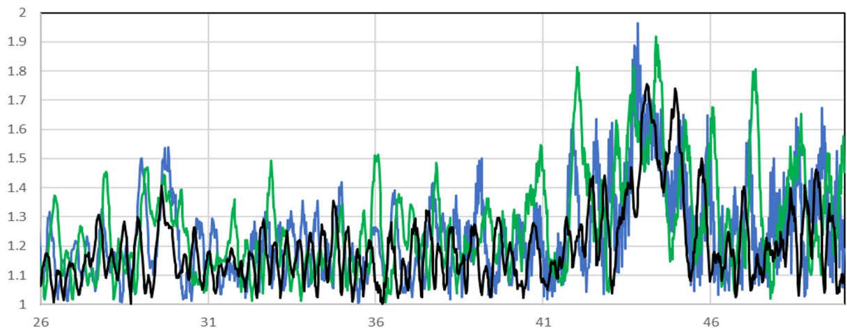
Figure 3. VSWR vs. frequency (26 to 50 GHz), 1a. standard path, 10 dB attenuation, measured on 3 units
