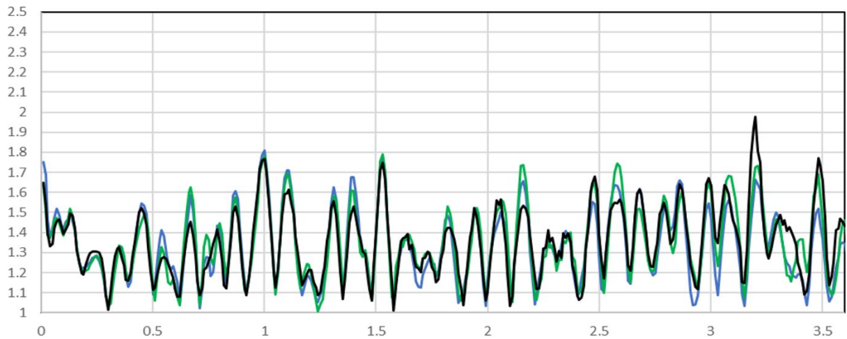
Figure 4. VSWR vs. frequency (0 to 3.5 GHz), 1c. preamp on, 0 dB attenuation, measured on 3 units
