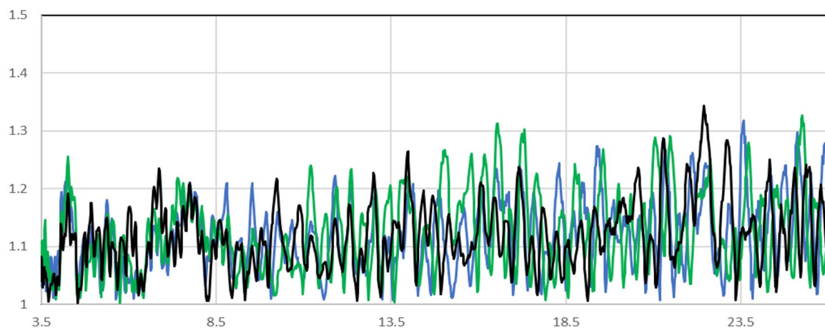
Figure 2. VSWR vs. frequency (3.5 to 26 GHz), 1a. Standard Path, 10 dB attenuation, measured on 3 units
