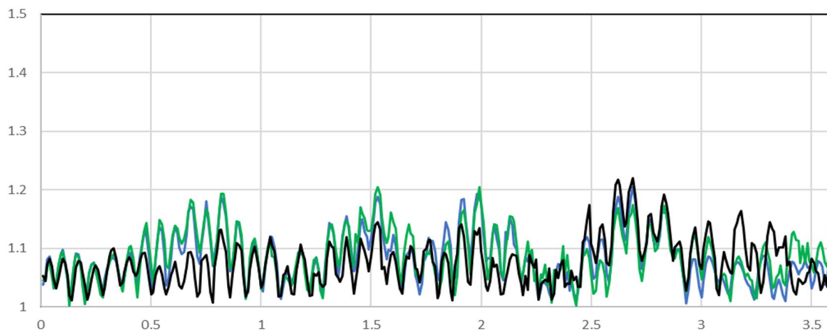
Figure 1. VSWR vs. frequency (0 to 3.5 GHz), 1a. Standard Path, 10 dB attenuation, measured on 3 units
