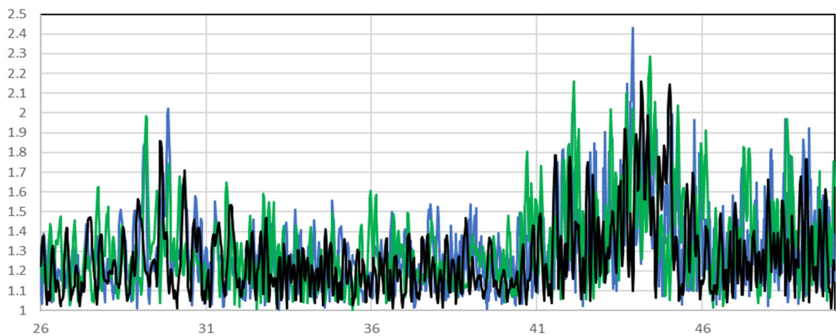
Figure 6. VSWR vs. frequency (26 to 50 GHz), 1c. preamp on, 0 dB attenuation, measured on 3 units
