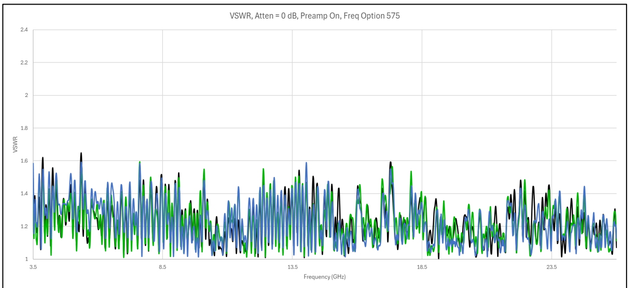
Figure 12. VSWR vs. frequency (3.5 to 26 GHz), 1c. preamp on, 0 dB attenuation, measured on 3 units
