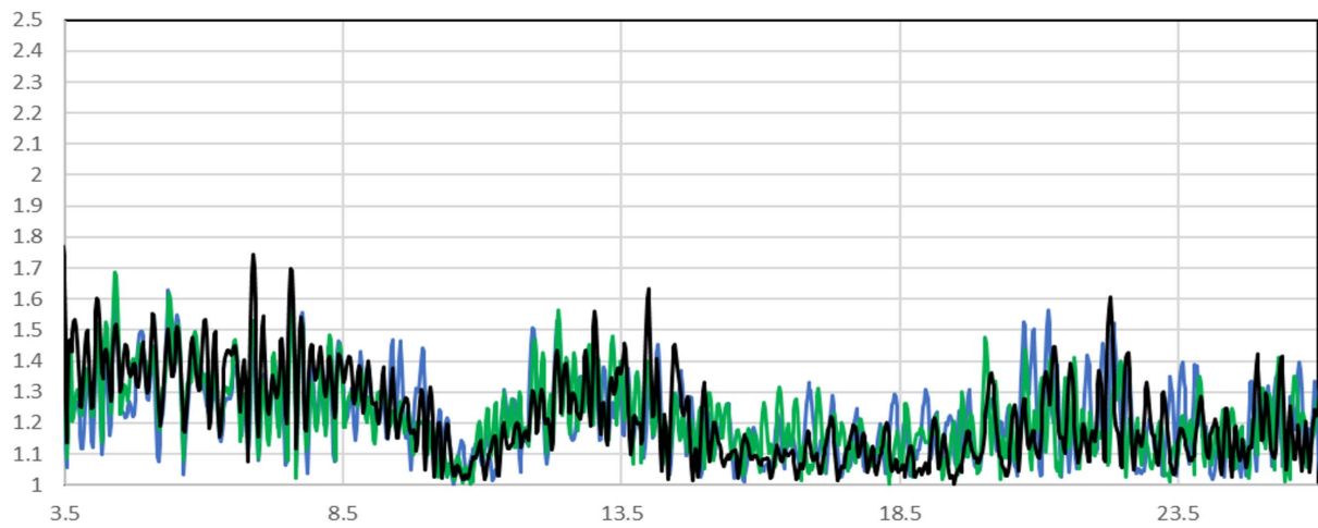
Figure 5. VSWR vs. frequency (3.5 to 26 GHz), 1c. preamp on, 0 dB attenuation, measured on 3 units
