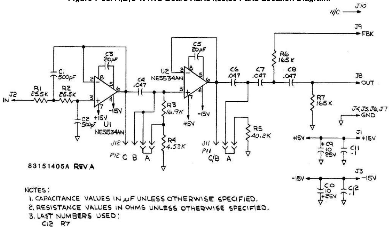
Figure 7-39. A,B,C WTNG Board A1A34,35,36 Schematic.
