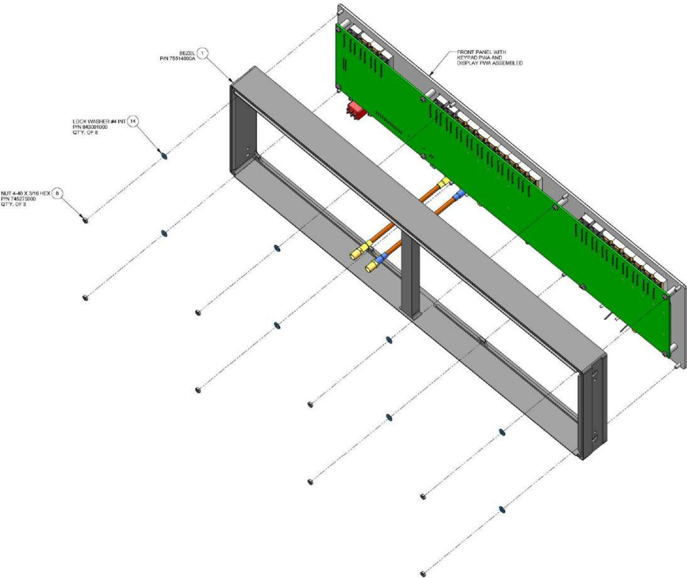
Figure 6-11. Front Bezel Assy (A17)
