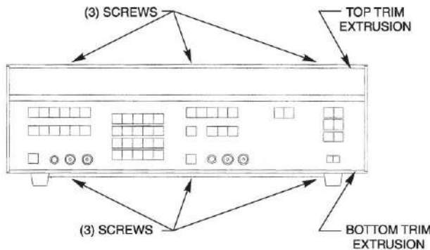
Figure 5-2. Removing Top and Bottom Trip Extrusions
