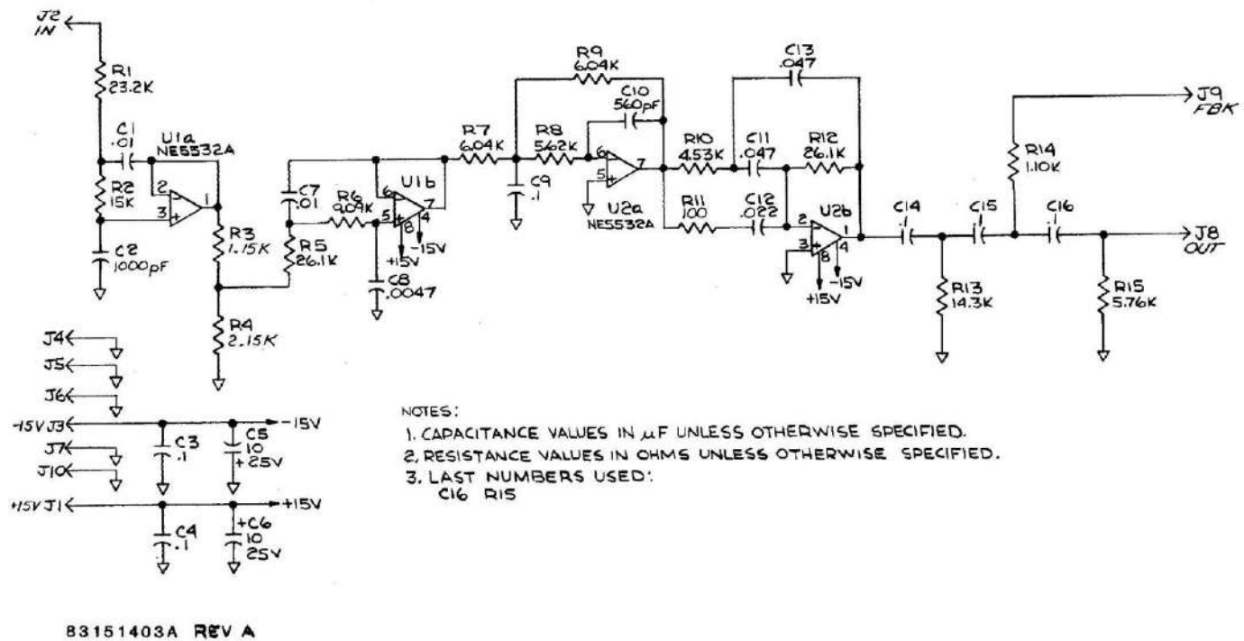
Figure 7-35. CCITT Board A1A31 Schematic.
