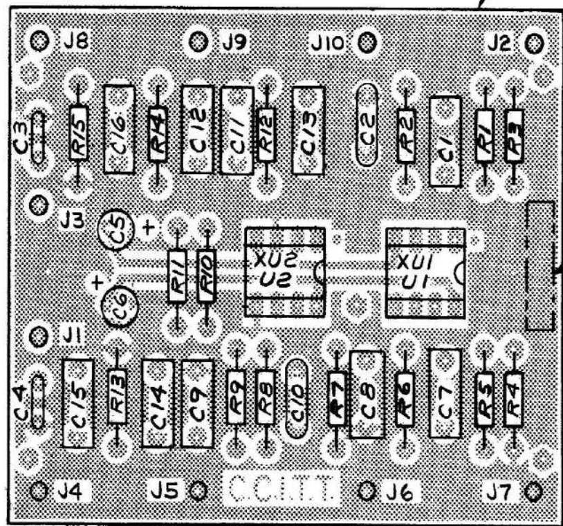
Figure 7-34. CCITT Board A1A31 Parts Location Diagram.
