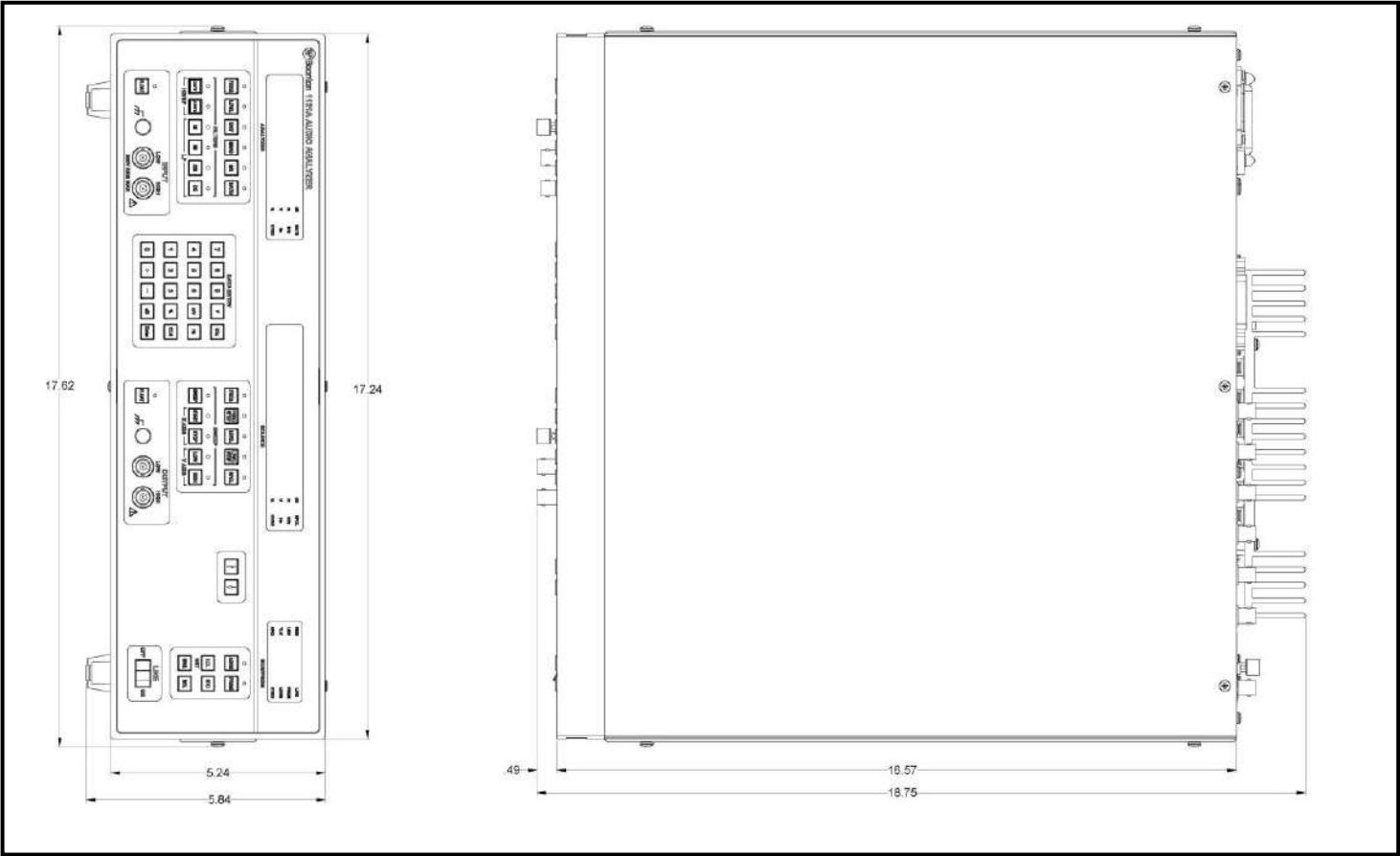
Figure 1-1. Outline Dimensions.
