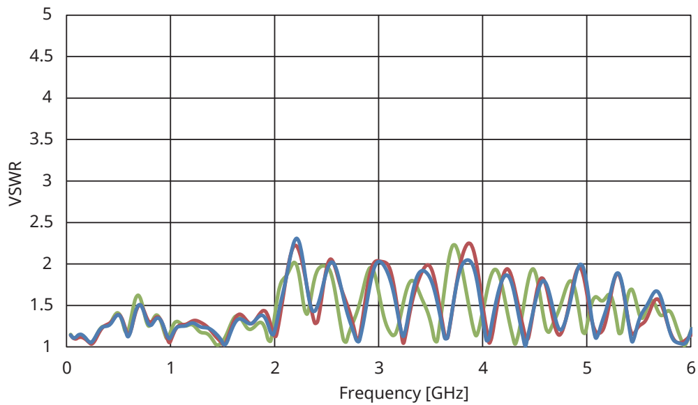
VSWR (meas.) (ATT: 0 dB, Preamp: On, \leq 6 GHz, 3 Units)
