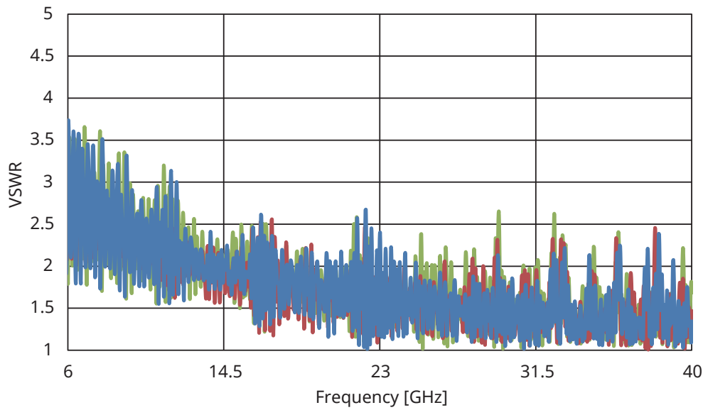
VSWR (meas.) (ATT: 0 dB, Preamp: Off, > 6 GHz, Microwave Preselector Bypass: Off, 3 Units)
