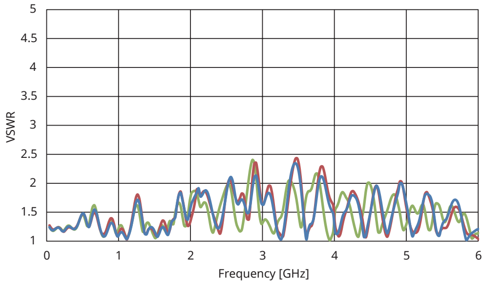
VSWR (meas.) (ATT: 0 dB, Preamp: Off, ≤ 6 GHz, 3 Units)
