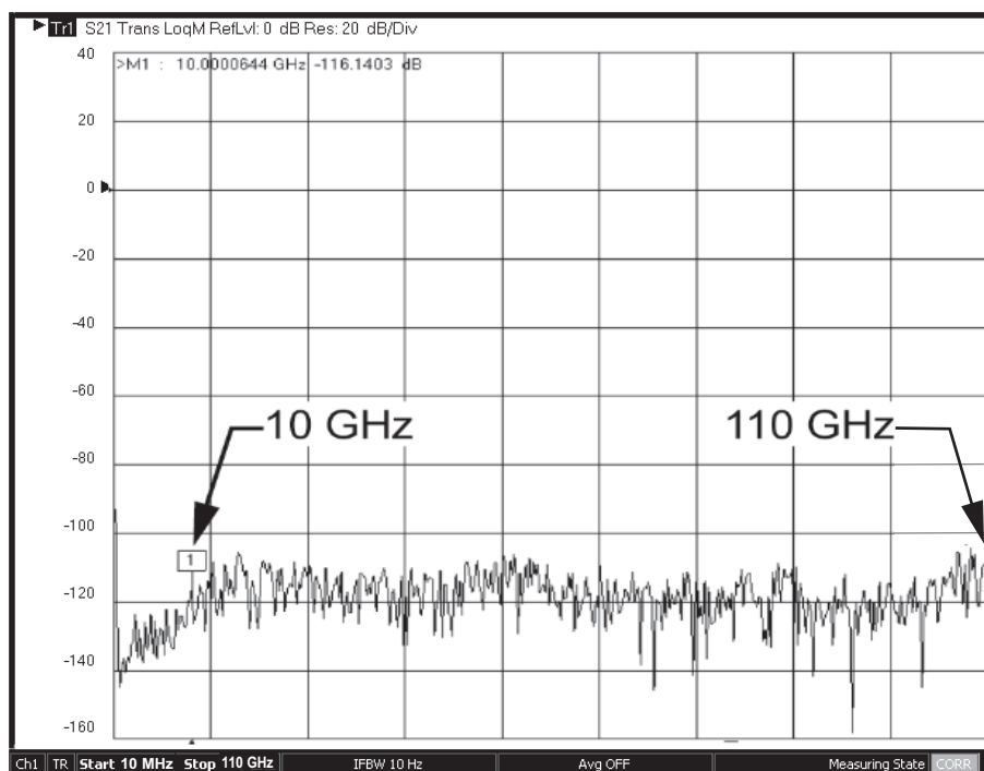
ME7838EX (Typical)
