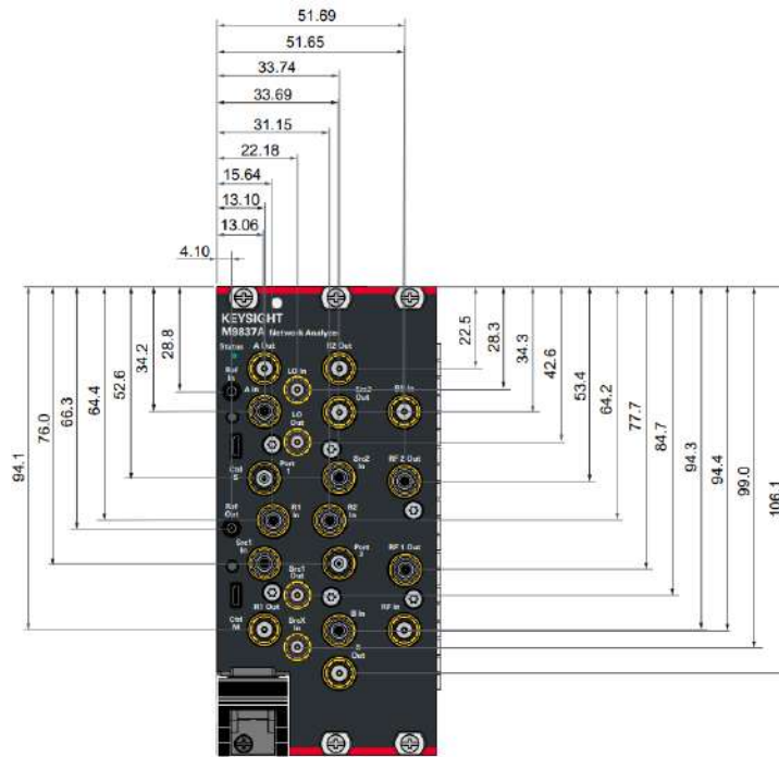
Dimensions (front view, M9834A with option 270, M9837A with option 205/270, in millimeters)
