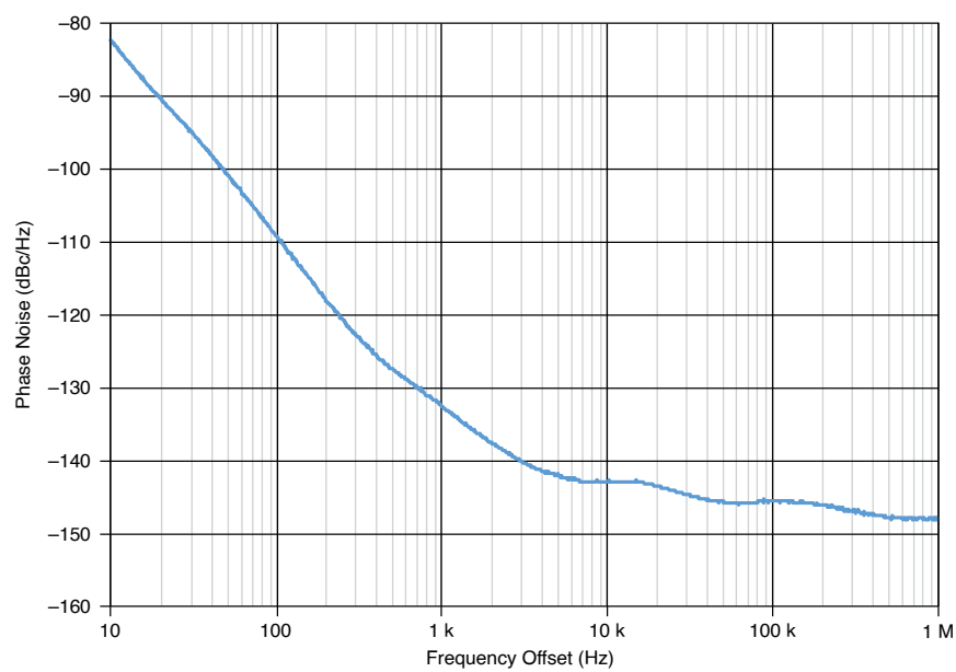
Figure 5. Phase Noise, Measured
