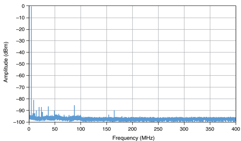
Figure 2. 5 MHz Spectrum at 0.6 V pk-pk , Measured
