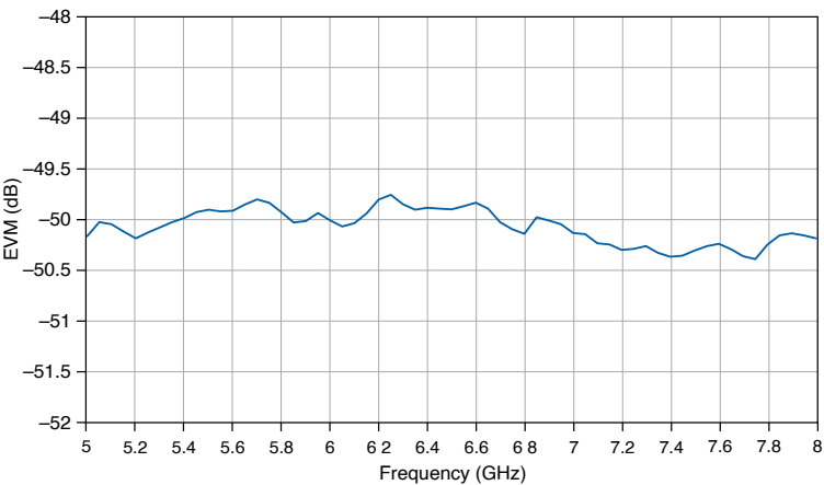
Figure 29. WLAN 802.11ax RMS EVM Versus Frequency, Nominal
