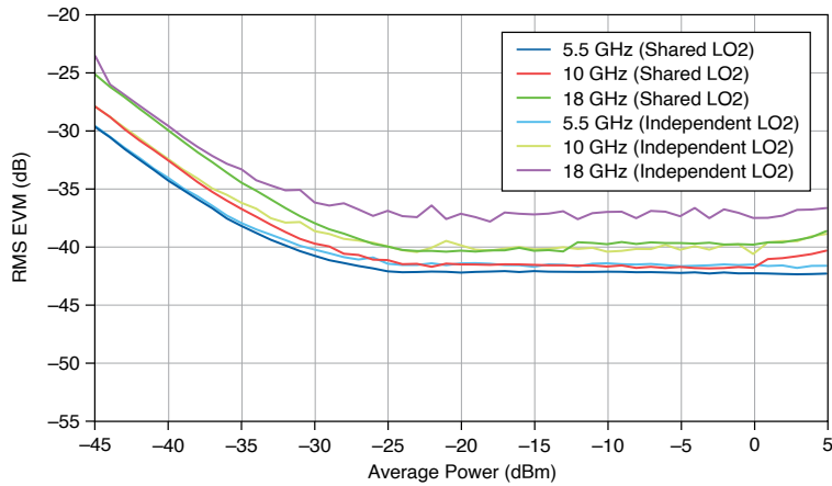
Figure 37. IF 5G NR RMS EVM versus Frequency (Shared LO2), Measured
