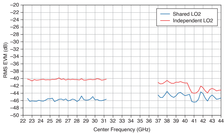
Figure 41. Direct TRX to Direct TRX RF 5G NR RMS EVM versus Frequency, Measured
