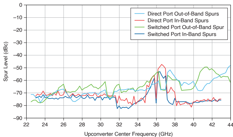
Figure 16. RF TRX Output Residual Spurs (Out-of-band and In-band) vs Upconverter Center Frequency, Measured
