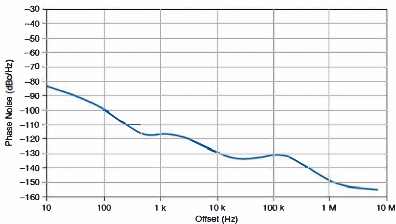
Figure 48. PXle-5653 Phase Noise, Measured (Spurs Not Shown)
