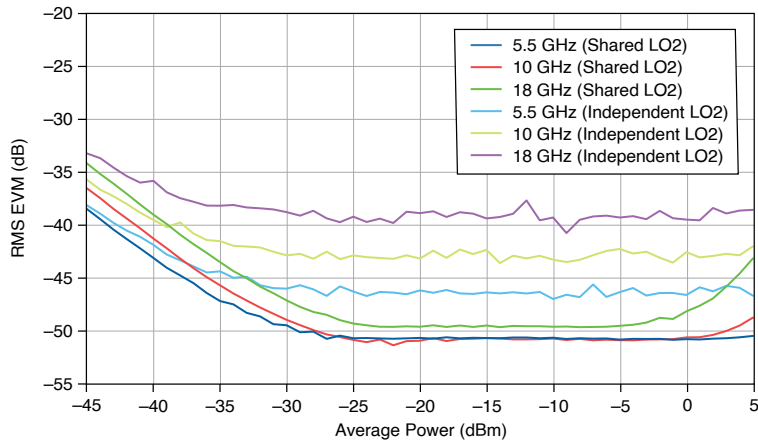
Figure 34. IF 5G NR 2 CC x 100 MHz RMS EVM versus Average Power, Measured
