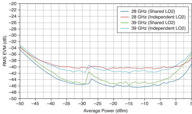
Figure 40. Switched to Switched RF 5G NR 1 CC x 100 MHz RMS EVM versus Average Power, Measured
