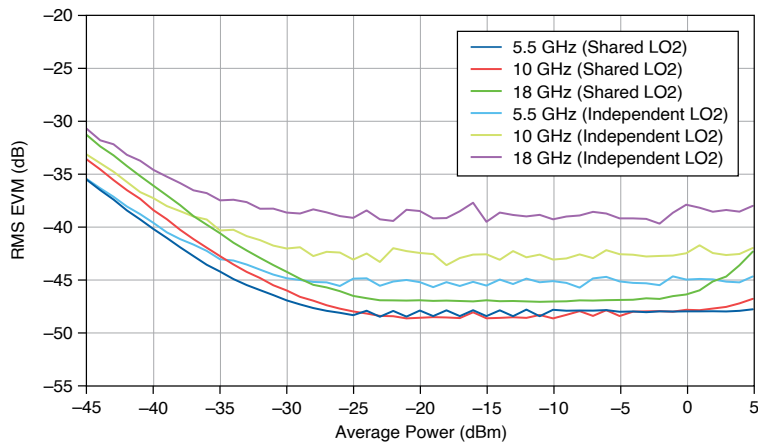
Figure 35. IF 5G NR 1 CC x 400 MHz RMS EVM versus Average Power, Measured
