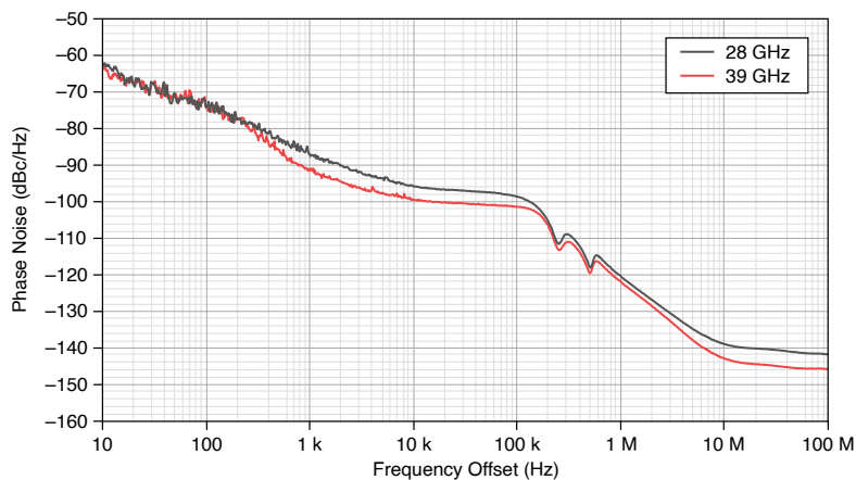
Figure 2. Onboard LO1 Phase Noise at 28 GHz and 39 GHz, Measured (Spurs Not Shown)
