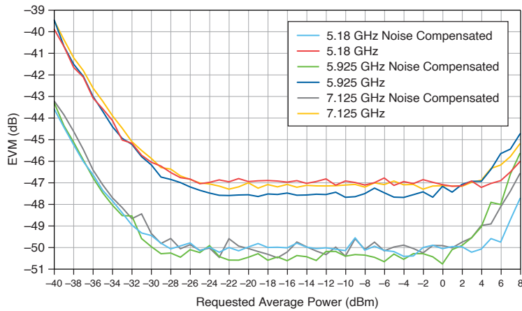
Figure 32. WLAN 802.11ax 80 MHz RMS EVM Versus Average Power (Loopback vs IF Out EVM), Measured
