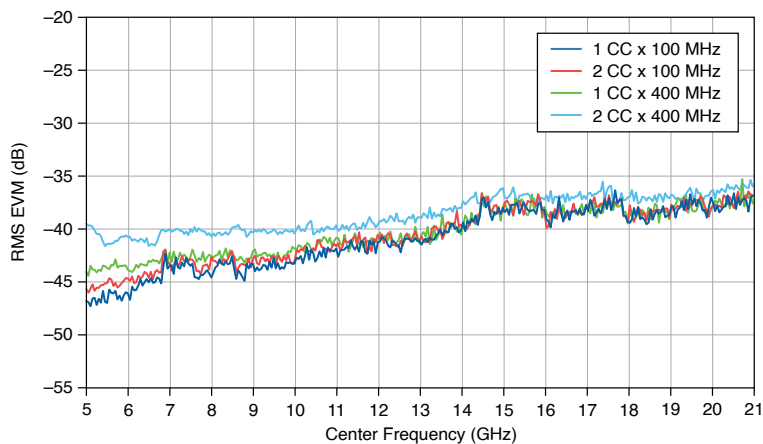
Figure 38. IF 5G NR RMS EVM versus Frequency (Independent LO2), Measured
