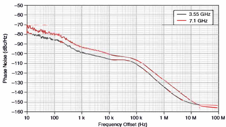
Figure 49. PXle-3622 Internal LO1 VCO Phase Noise, Measured (Spurs Not Shown)
