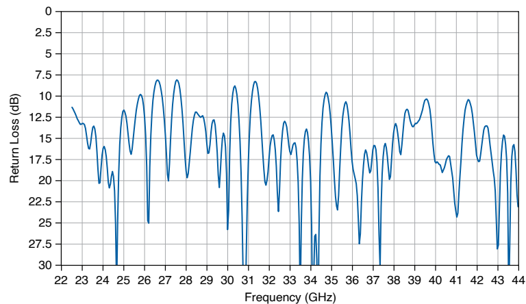
Figure 44. mmRH-5582 RF Input Port Return Loss, Measured at Direct TRX Port
