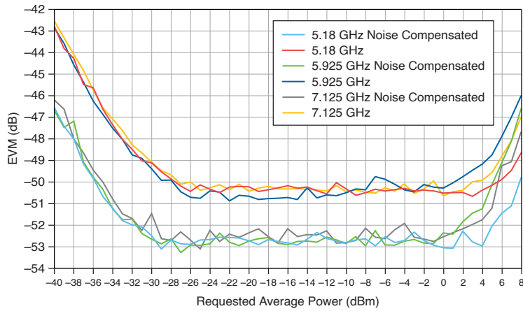
Figure 31. WLAN 802.11ax 160 MHz RMS EVM Versus Average Power, Measured
