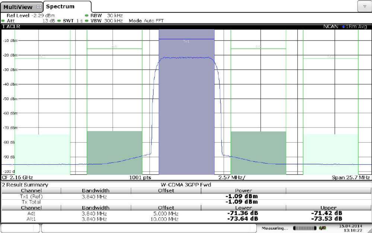
Digital standard 3GPP FDD test model 1, 64 DPCHs ACLR (meas.)
