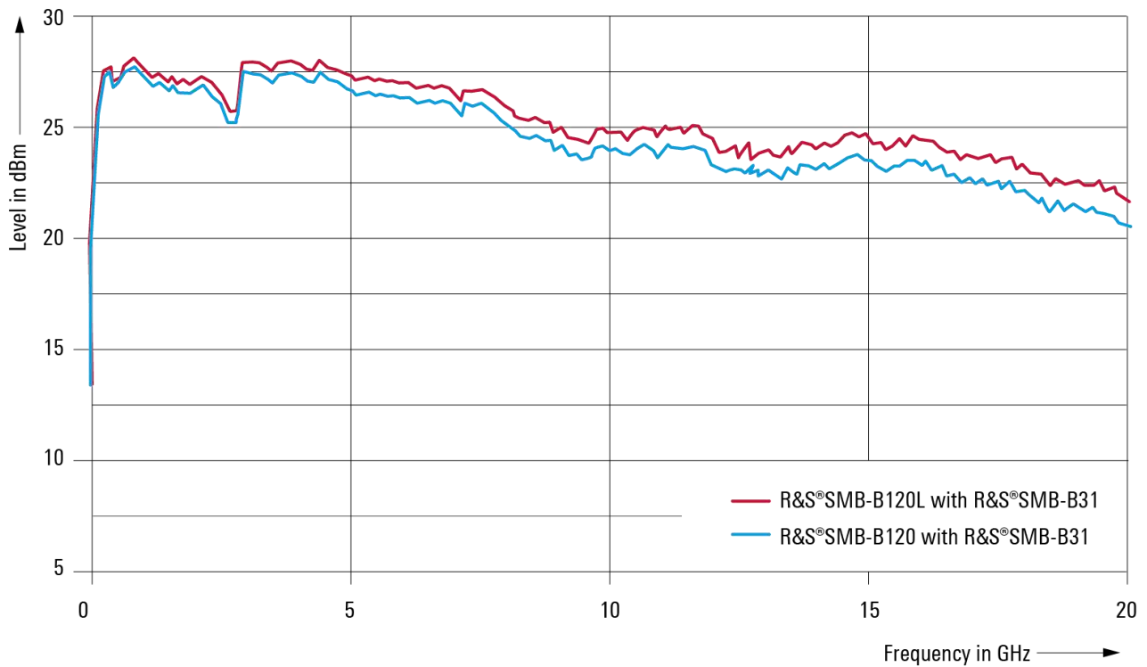
Maximum available output level versus frequency (meas.)
