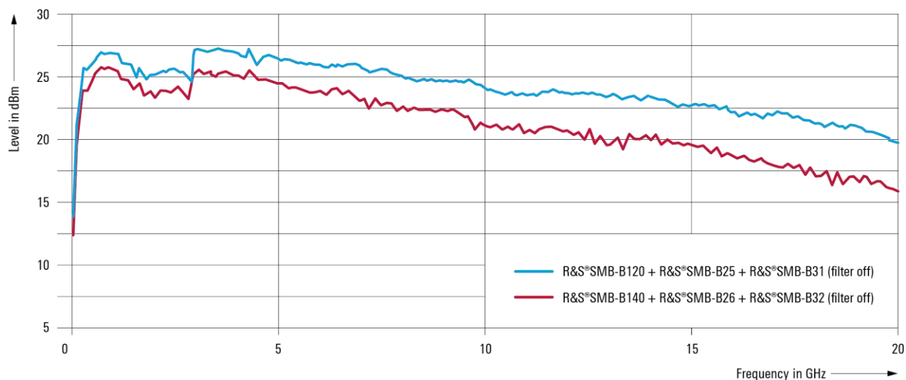
Maximum available output level versus frequency, low harmonic filter off (meas.)
