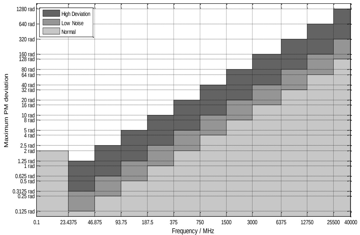
\phi M deviation versus frequency and operating mode
