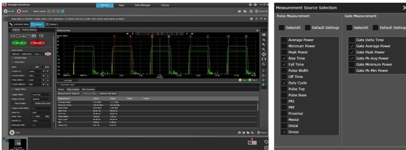
Figure 8. Multi-channel trace display with 4-pairs of gates and automatic pulse parameters measurement (sample screen shot with two X-Series power sensors)
