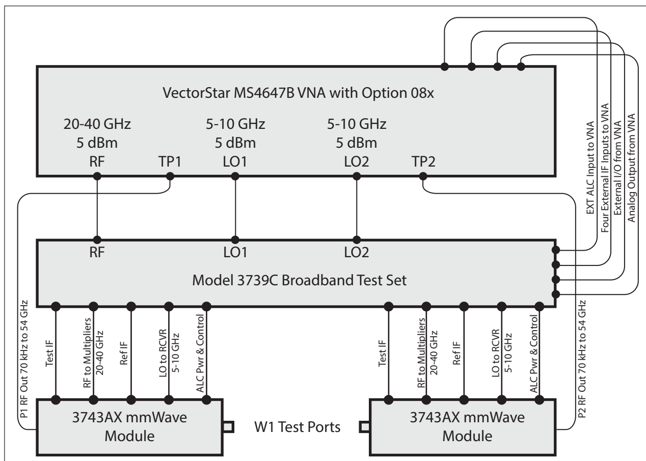
ME7838AX 2-port Broadband System
