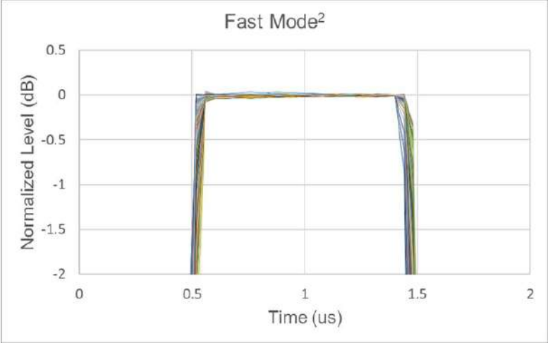
2. Measured with a 15 MHz IF bandwidth, averaging factor of 16 (Average Type = Point). With 1 \mu s pulse width setting. 500 ns/div.
