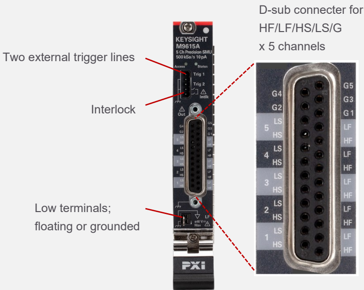
Figure 1. Front panel
