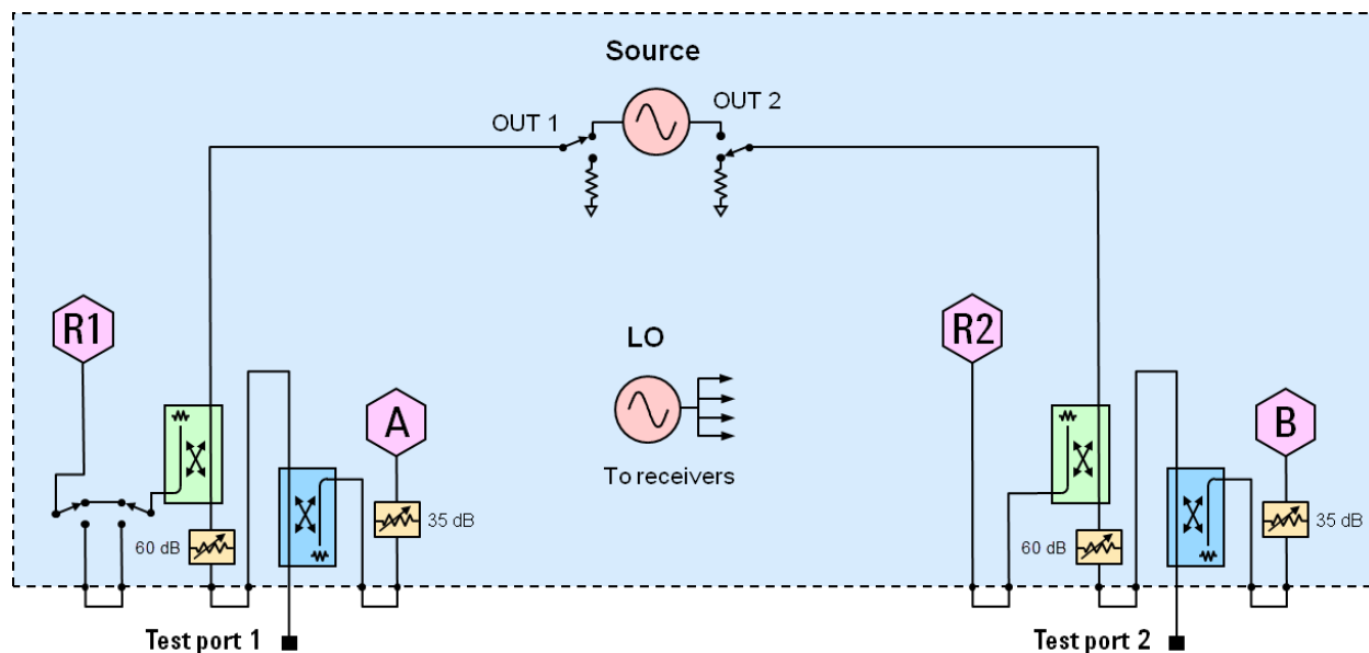
Figure 2. 2-Port N5244B and N5245B Option 217
