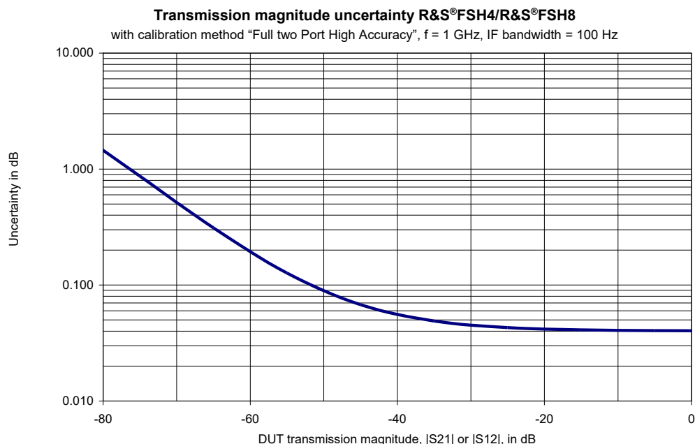
Transmission magnitude uncertainty, R&S®FSH4/R&S®FSH8 with the R&S®FSH-K42/R&S®FSH-K45 option
