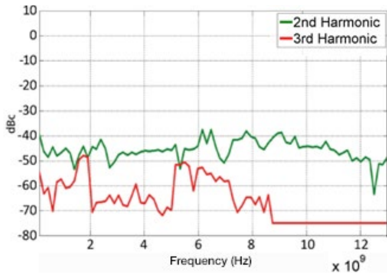
Figure 6. Typical harmonics
