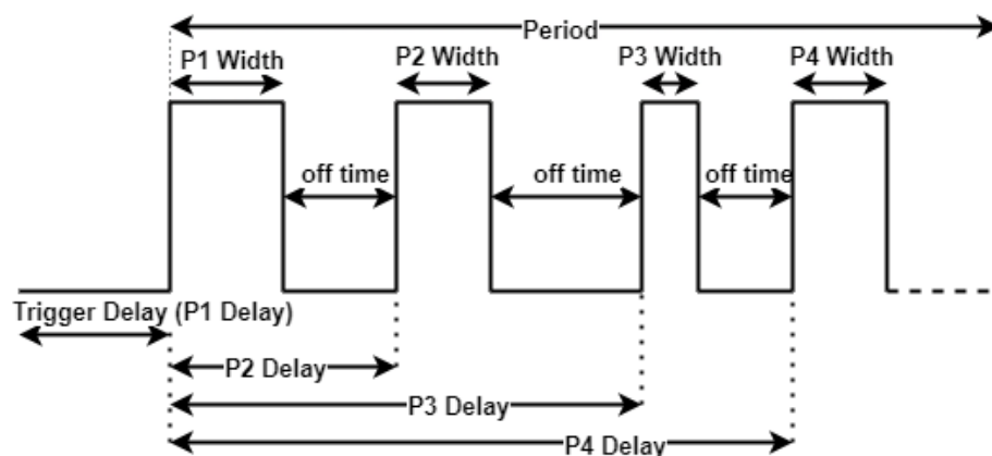
Figure 8. N-Pulse modulation
