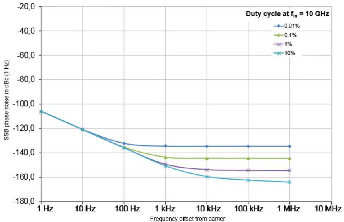
Typical AM noise sensitivity at f_{in} = 10 GHz (start offset = 1 Hz, correlation factor = 1, signal level = 10 dBm, gating = on)
