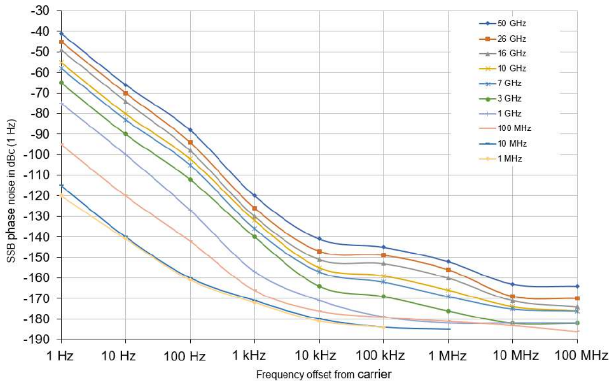
Typical phase noise at different center frequencies with R&S®FSWP-B60 option (start offset = 1 Hz)
