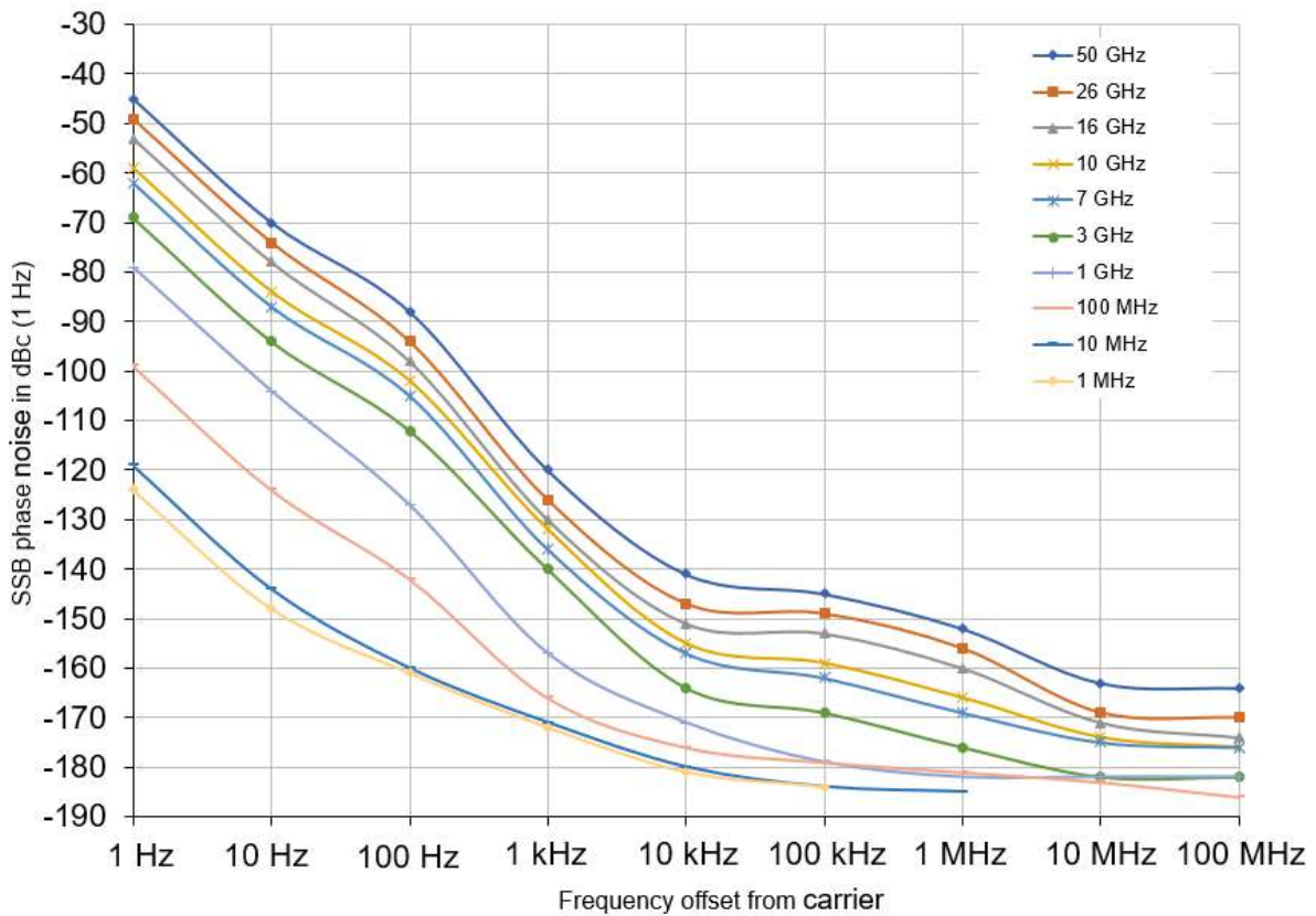
Typical phase noise at different center frequencies with R&S®FSWP-B60 and R&S®FSWP-B4 options (start offset = 1 Hz)
