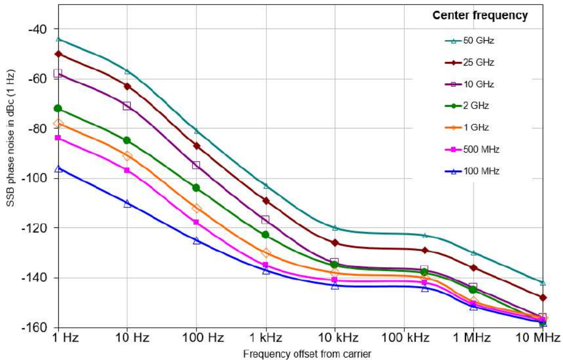
Typical phase noise at different center frequencies in spectrum analyzer mode (with R&S®FSWP-B4 option for offsets \leq 10 Hz)
