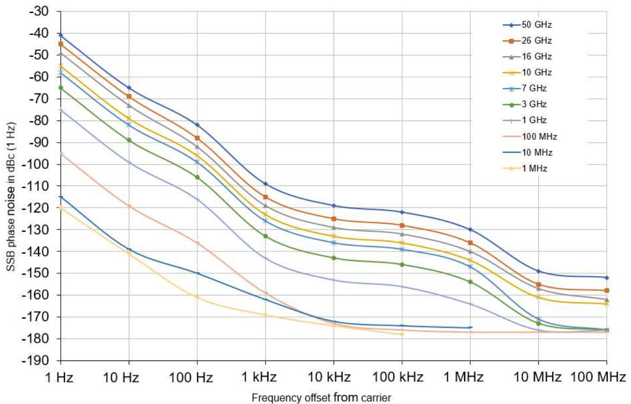
Typical phase noise at different center frequencies with R&S®FSWP-B4 option
