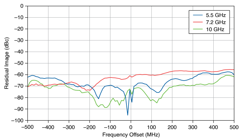
Figure 6. IF Output Residual Sideband Image, 0 dBm Peak Power, Measured
