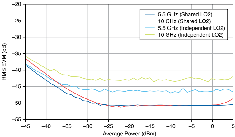
Figure 15. IF 5G NR 1 CC x 100 MHz RMS EVM versus Average Power, Measured
