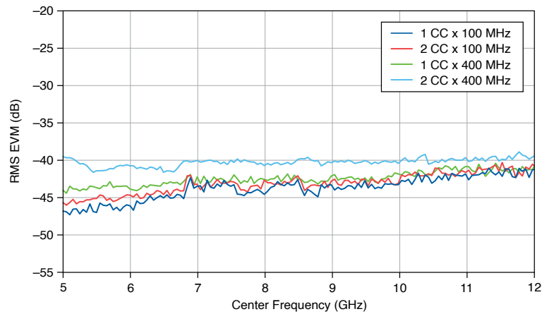
Figure 20. IF 5G NR RMS EVM versus Frequency (Independent LO2), Measured
