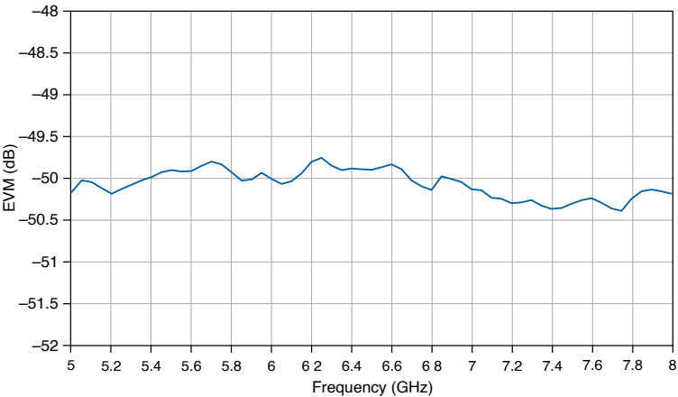
Figure 14. WLAN 802.11ax RMS EVM Versus Frequency, Nominal
