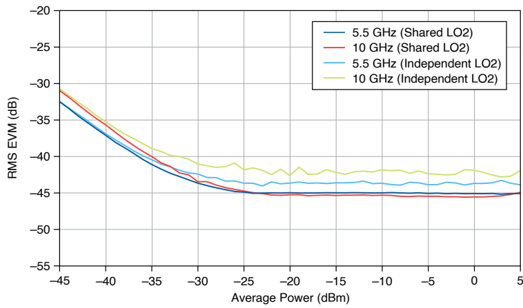
Figure 18. IF 5G NR 2 CC x 400 MHz RMS EVM versus Average Power, Measured
