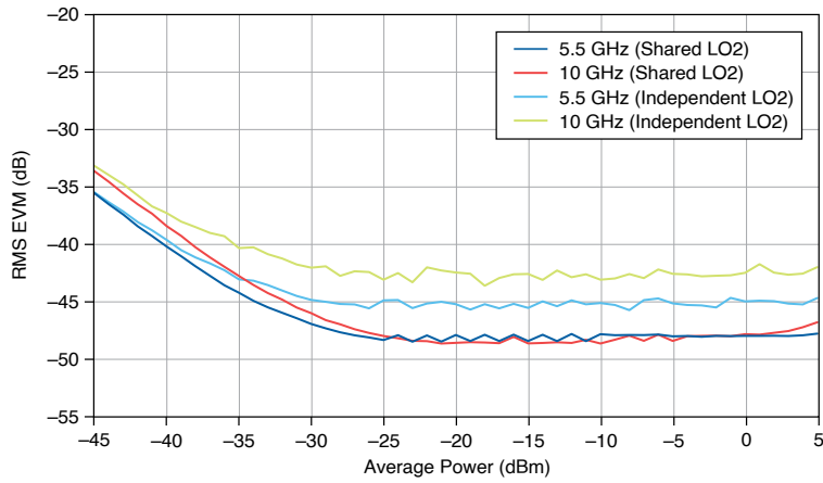
Figure 17. IF 5G NR 1 CC x 400 MHz RMS EVM versus Average Power, Measured
