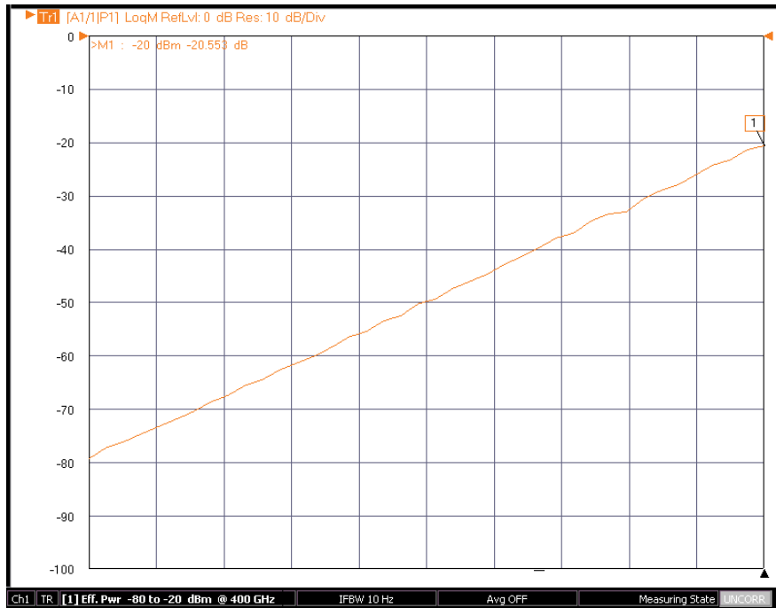
Real time power sweep of VDI WR2.2 module using system power level OFF control and no mechanical attenuators.
