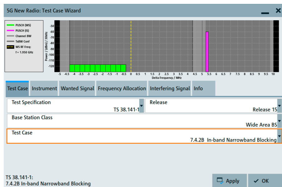
The 5G NR test case wizard allows the R&S®SMW200A to be configured conveniently and cleverly for BTS tests in line with 3GPP TS38.141. The wanted signal and interferer for a narrowband blocking test are set.
