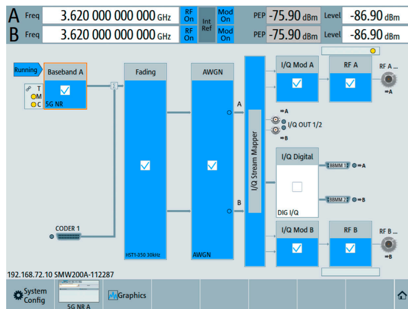
The R&S®SMW200A is perfect for 5G NR base station performance tests in line with 3GPP TS38.141. The block diagram (left) and fading settings (below) for testing with high speed train fading are shown.
