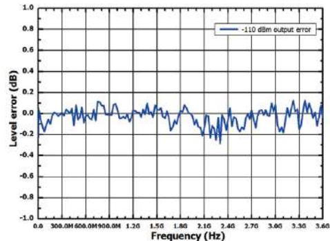
Measured at -110 dBm,level error vs.frequency
