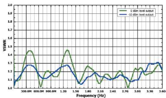
Measured VSWR vs.frequency
