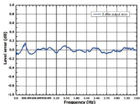
Measured at 0 dBm,level error vs.frequency
