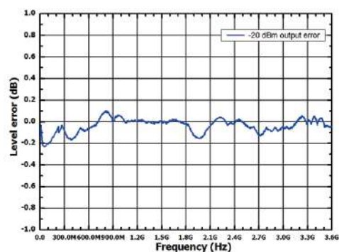
Measured at -20 dBm,level error vs.frequency
