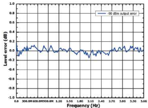
Measured at -90 dBm,level error vs.frequency
