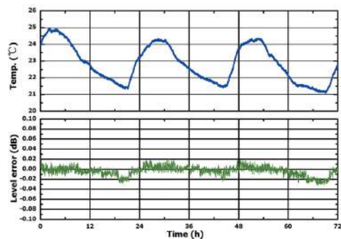
Measured level repeatability @ 1 GHz,0 dBm
