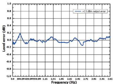
Measured at +13 dBm,level error vs.frequency
