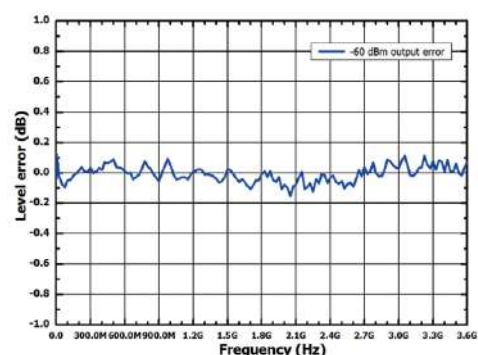
Measured at -60 dBm,level error vs.frequency
