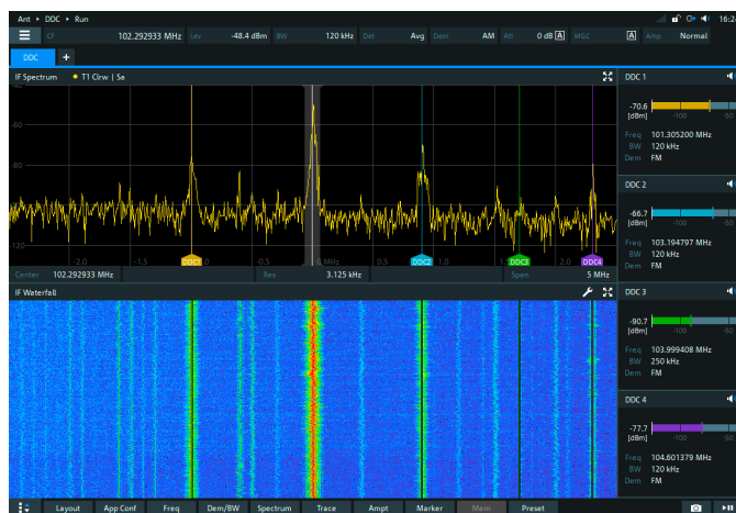
Monitoring with up to 4+1 demodulation channels with different parameters in the real-time bandwidth
