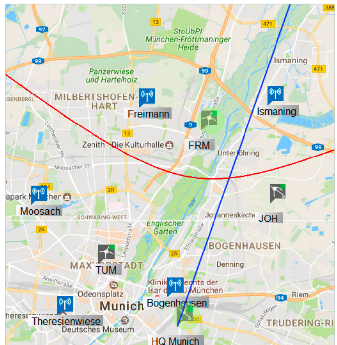
Hybrid TDOA/AOA location result in R&S®ARGUS. Combined with data from spectrum management, it shows that the measured location of the interferer does not coincide with a licensed transmitter.
