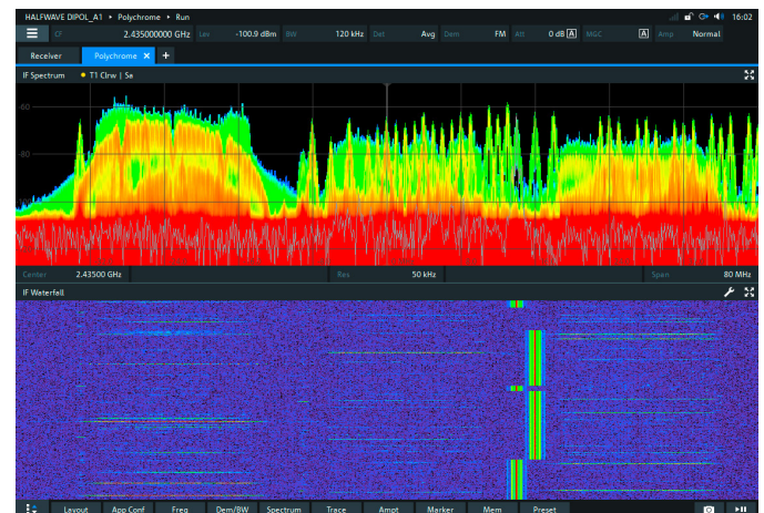
Polychrome spectrum uses color coding to indicate the relative level occupancy over time
