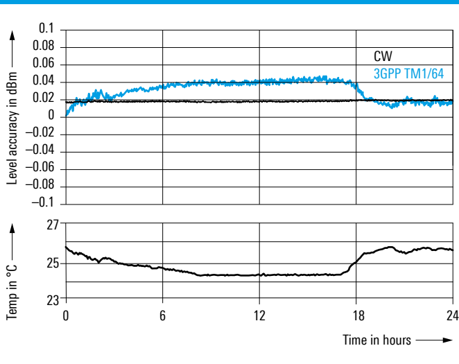
Level repeatability for a 3GPP TM1/64 signal with a crest factor of 10.55 dB, at 5 dBm (measured)
