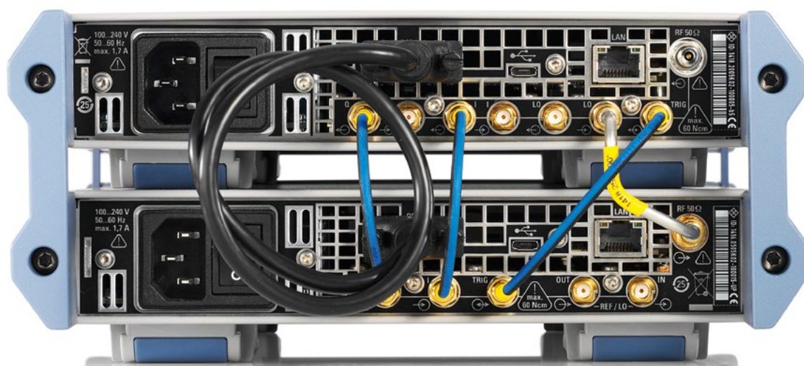
Connections between the R&S®SGS100A and the R&S®SGU100A.
