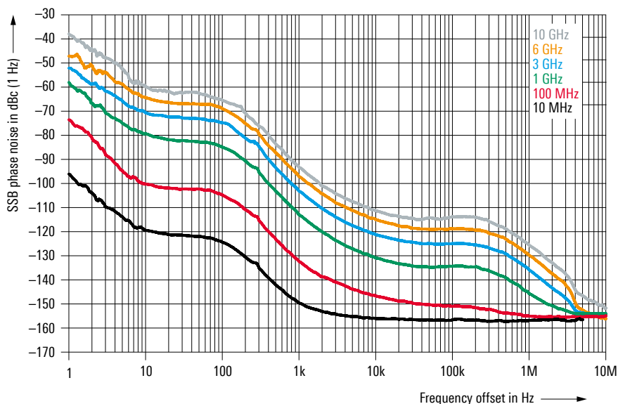
SSB phase noise of the R&S®SGS100A with R&S®SGS-B1 internal OCXO option (measured)
