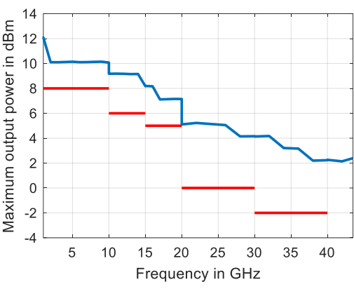
Typical maximum output power in dBm versus frequency of the R&S®ZNB43
