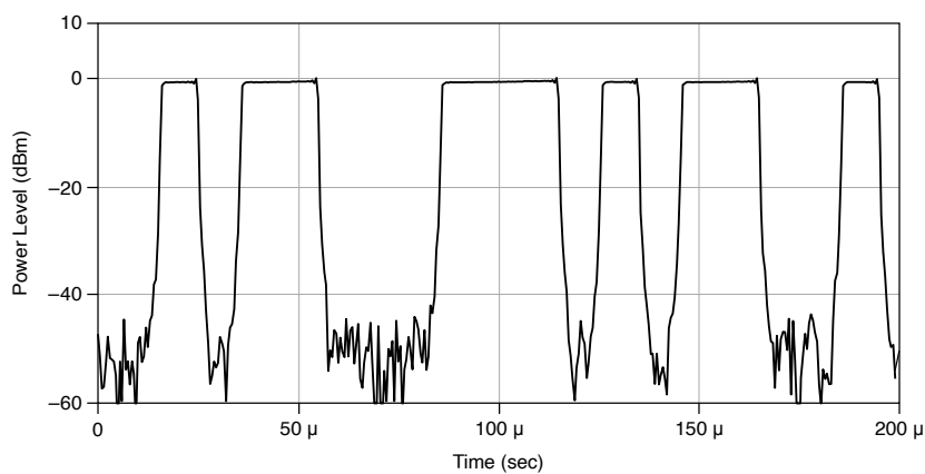
Figure 15. OOK Diagram, 1.0 GHz Carrier, 100 kHz Symbol Rate, Ninth-Order PRBS
