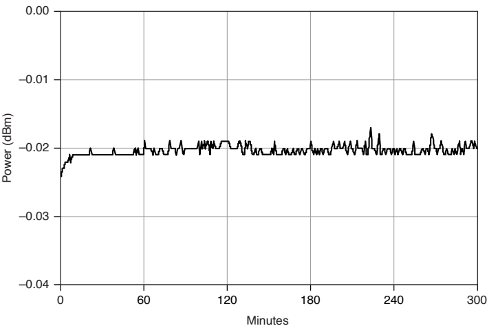
Figure 11. Typical Power (0 dBm) at 2.4 GHz Over Time 6
