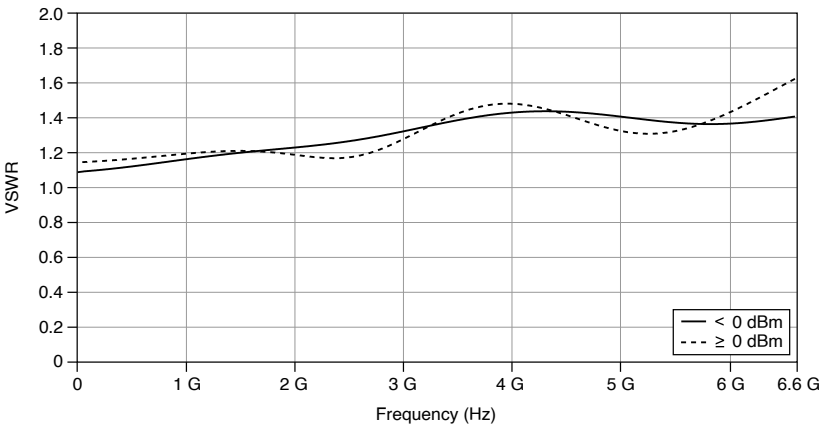
Figure 1. Measured VSWR
