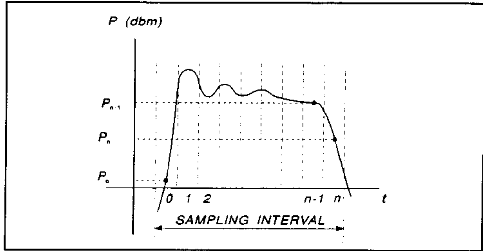
Figure 5-7. Sampling Intervals
